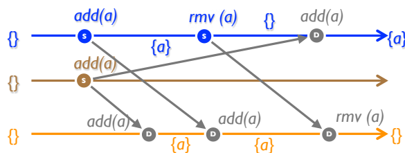
Figure 11: Counter-example: Set with concurrent add and remove (op-based)
