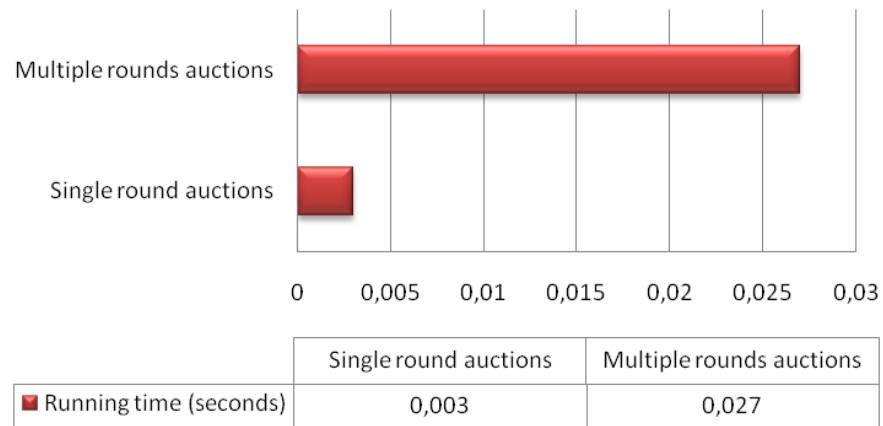
Fig.7. Comparison between the two algorithms in terms of running time
