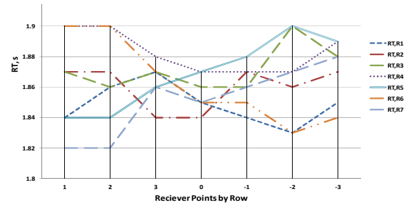
Figure 16. RT for the square mosque geometry at 1kHz as a function of worshippers rows (Imam position).
