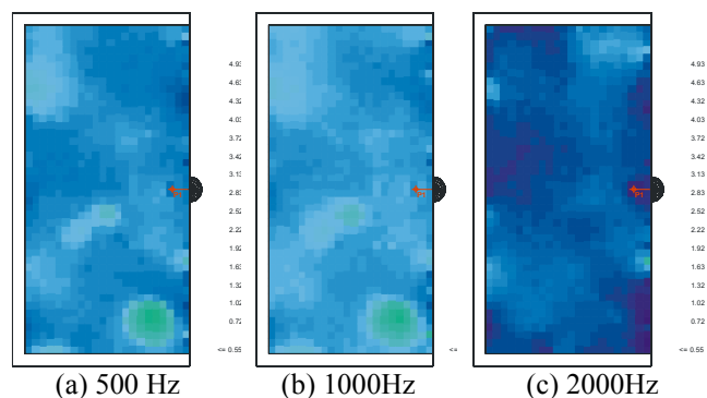
Figure 5. RT for the 1:2 rectangular mosque geometry, when the mosque is assumed empty, a: at 500Hz, b: at 1kHz, and c: at 2kHz (Imam position).
