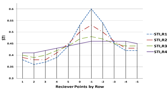
Figure 14. STI for the 1:2 rectangular mosque geometry as a function of worshippers rows (Khatib position).
