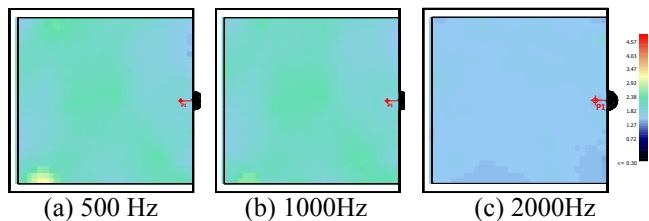
Figure 15. RT for the square mosque geometry; a: at 500Hz, b: at 1kHz, and c: at 2kHz (Imam position).
