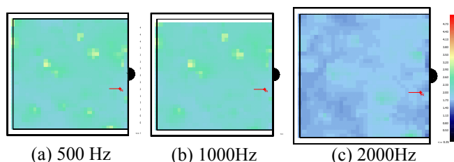
Figure 22. EDT for the square mosque geometry; a: at 500Hz, b: at 1kHz, and c: at 2kHz (Khatib position).
