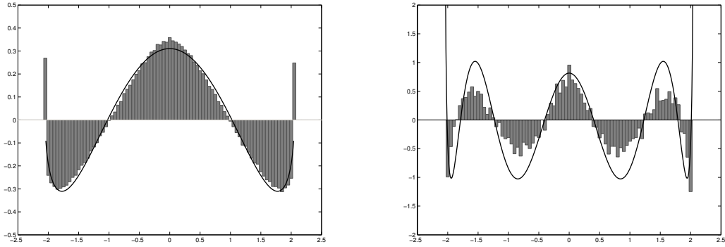
Figure 5: Left: Histogram of c\left(\mu_n^c - \Lambda_{1+\frac{1}{2c}}(\sigma)\right) compared with the density of \Lambda_{1+\frac{1}{2c}}\left(\hat{\sigma}^{\{1\}}\right) . Right: Histogram of c^2\left(\mu_n^c - \Lambda_{1+\frac{1}{2c}}\left(\sigma + \frac{1}{c}\hat{\sigma}^{\{1\}}\right)\right) compared with the density of \Lambda_{1+\frac{1}{2c}}\left(\hat{\sigma}^{\{2\}}\right) .
