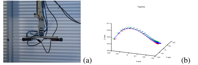
Fig. 5. (a) The non-overlapping stereo eye-in-hand configuration attached to INRIA's 6dof Afma 6 robot. (b) A 3D trajectory of the robot performing visual servoing from (12). A video of the experiment is available accompanying this paper.
