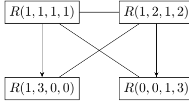
Figure 8: The prioritized conflict graph G(I_4, F_4, >_4) .
