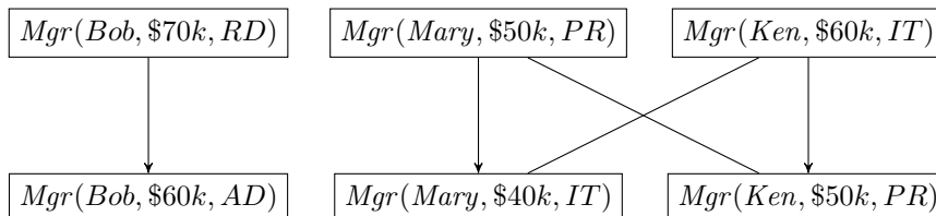
Figure 6: Prioritized conflict graph from Example 2.
