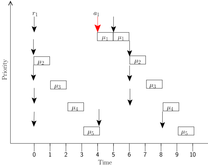
Figure 2. Example of how the WCRT of a lower priority message \mu_5 is affected by the additional jitter caused by priority inversion that is suffered by a higher priority message \mu_1 .
