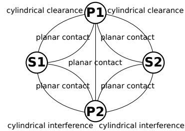
Figure 11: The CIG resulting from the two threaded connections configuration.
