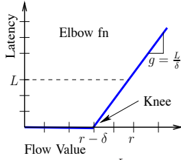
Fig. 2. Link latency function: L_2(x) = \frac{L}{\delta}(x - r) + L , for r - \delta \leq x and the parameters are: r = 1, L = 0.1, \delta = 10^{-3}, g = \frac{L}{\delta} = 100 .
