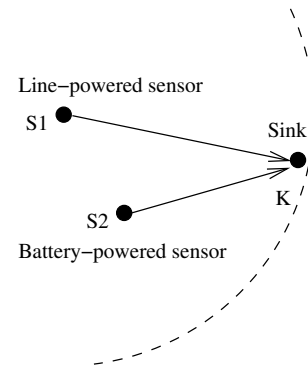
Fig. 2. Battery-powered sensor S_2 overhearing the packet of line-powered sensor S_1 destined to the sink K , d_{S_1 S_2} < d_{S_1 K}
