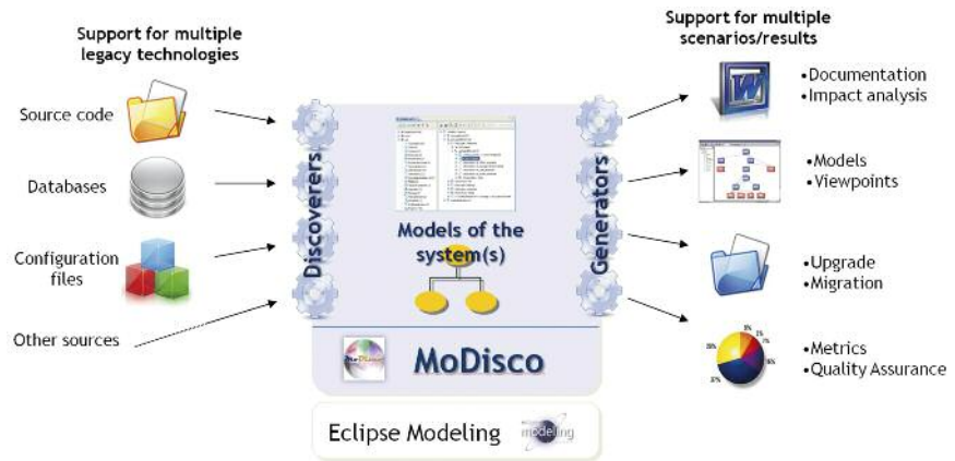
Figure 1: MoDisco, a Model Driven Reverse Engineering approach & framework
