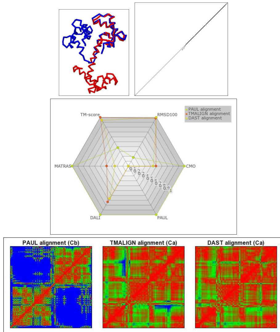
Figure 3: Top left: The two calmodulin conformers (PDB IDs 4cln and 2bbm) superpositioned according to the TM-alignment, which aligns only one of the two regions that move relative to each other. Top right: Comparison of the alignment traces. Each axis corresponds to one conformer. Black boxes denote residue pairs aligned by all three scorings, PAUL, TM-ALIGN and DAST. Light gray denotes residue pairs aligned by only one scoring. An intermediate shade of gray denotes agreement of two scorings. PAUL aligns all residues of the two conformers, TM-ALIGN and DAST the C-terminal region. Center: The radar chart illustrates the difference between scorings that are more in favor of a flexible alignment, i.e. CMO, PAUL, DALI and MATRAS, and scorings that are more in favor of a rigid superposition of low RMSD. Bottom: The distance difference matrices illustrate the difference between the flexible PAUL alignment, that aligns all residues in spite of large distance differences (colored blue), and the TM- and DAST alignment, which exclude large distance differences, but only align the C-terminal region.
