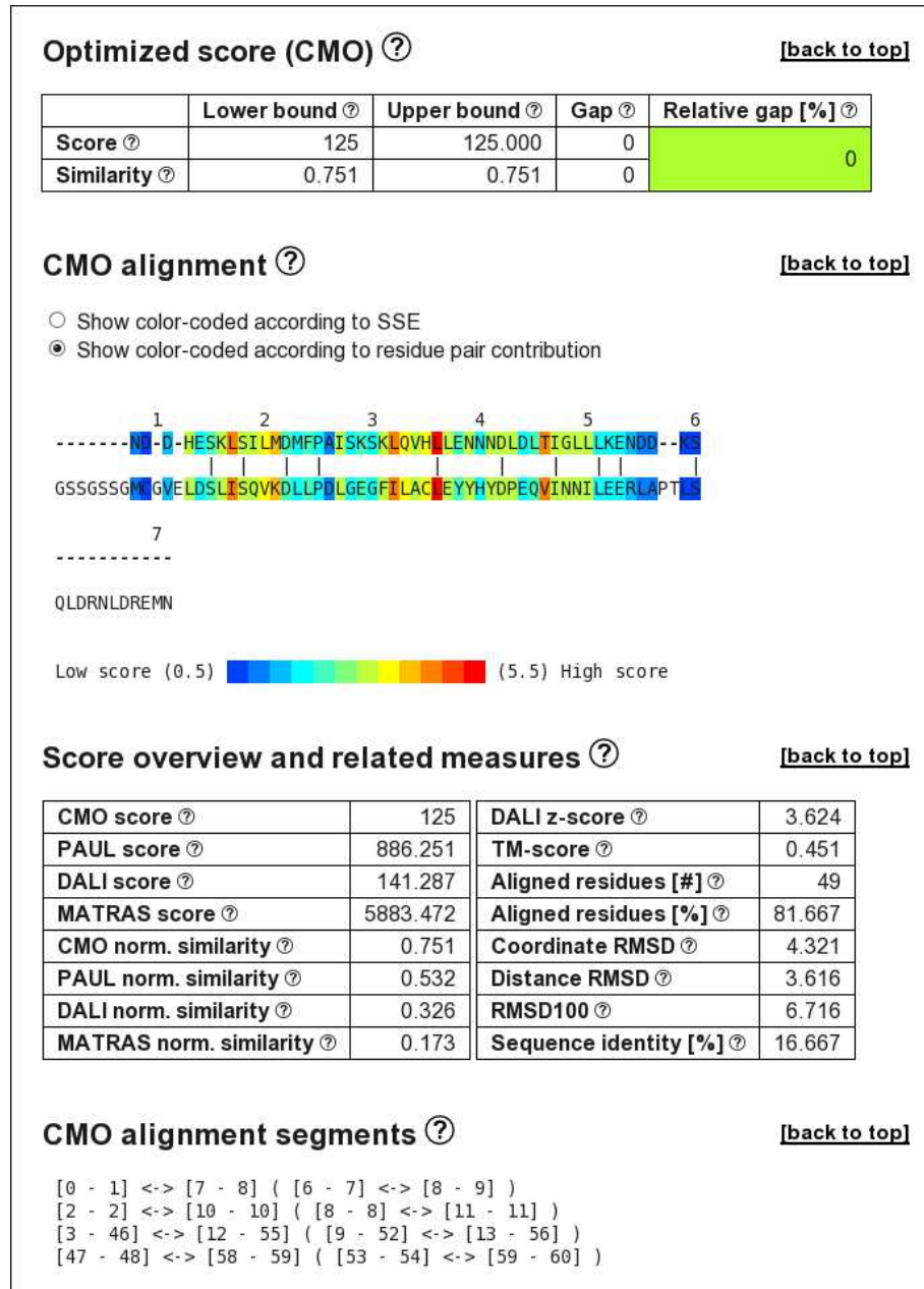
Figure 1: Parts of the information displayed on the website for the CMO alignment of lotrA and 2di0A.
