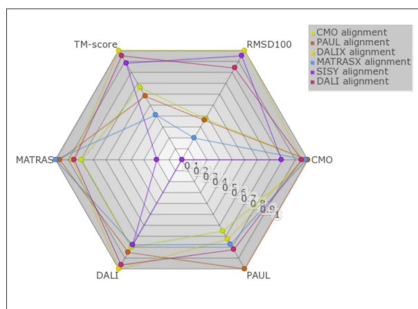
Figure 2: A radar chart for comparison of alignment scores for six different alignments of 1otrA and 2di0A. The closer a point is to 1, the better the corresponding score. CMO, PAUL, DALIX and MATRASX alignments have been computed by our exact algorithm and are provably optimal concerning their respective score. The SISY reference alignment aligns 38 residues of the CUE2 domain. The DALI alignment was computed by the DALI server and has slightly lower DALI score than the optimal DALIX alignment. The reference alignment is far behind in all scores except RMSD100 and TM-score, for which it performs quite well. The MATRASX alignment performs especially poor for these two measures. Intuitively, the DALIX alignment is most preferable since it has optimal DALI and close to optimal CMO, PAUL and MATRAS scores, as well as the best TM-score and RMSD100.
