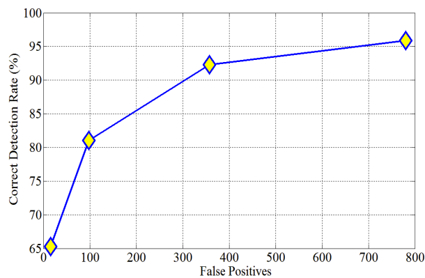
Figure 4. ROC curve for our face detector on the MIT+CMU test set. The detector was run once using a step size of 1.1 and starting scale of 1.25 (73,130,500 sub-windows scanned)
