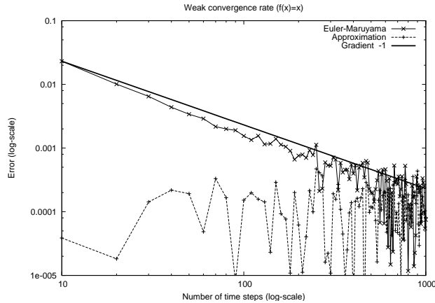
Figure 1: No. of time steps – weak error ( f(x) = x ).
