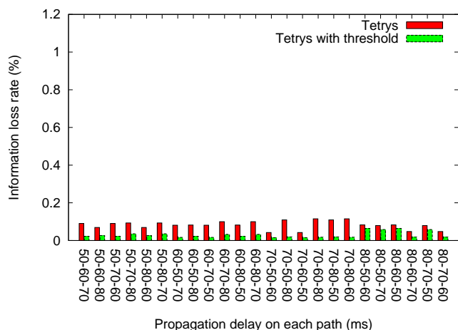
Fig. 9. Tetrys without threshold and with threshold \theta = 5\% at mean burst size of 2 packets
