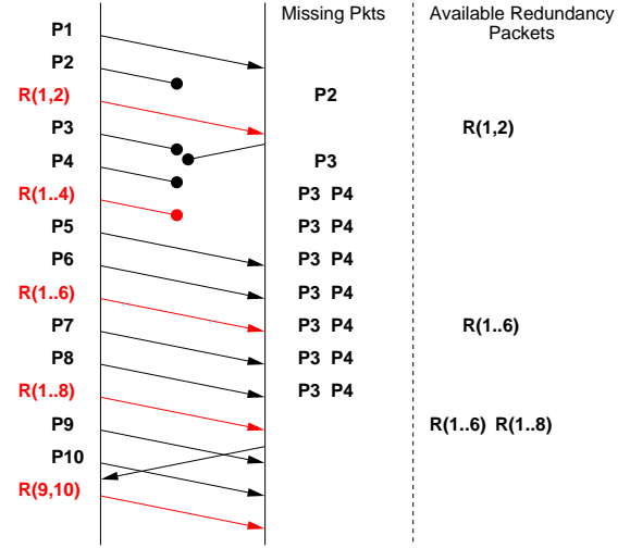
Fig. 2. A simple data exchange with Tetrys ( k=2 ) [10]
