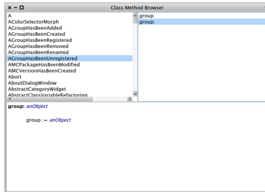
Figure 6: Our classes and method browser with a method selected
