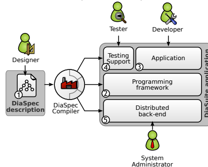
Figure 2: The DiaSuite tool-based development process
