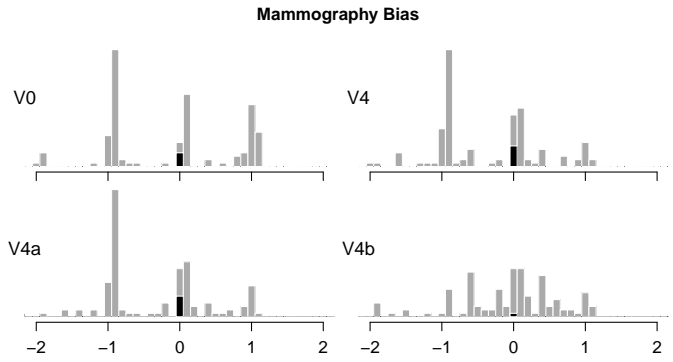
Fig. 4. Distributions of biases in answers to the mammography problem ( N = 120 each) per presentation type. Black bars are exact answers.
