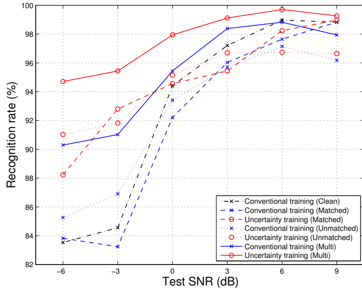
Figure 7: Average speaker recognition accuracy (in %) as a function of the test SNR for all training strategies and training conditions with the oracle diagonal uncertainty estimator. The results are averaged over the training SNRs corresponding to each training condition. Uncertainty decoding is performed in all cases.
