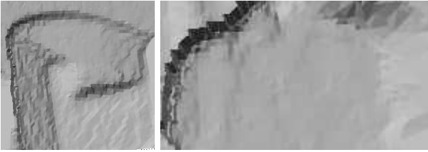
(a) Dense surface reconstruction using the disparity map D_p corresponding to a 2D triangulation of the TOF data points. Zoomed sofa chair and zoomed T-shirt from SET-2 in Fig. 7(a).
