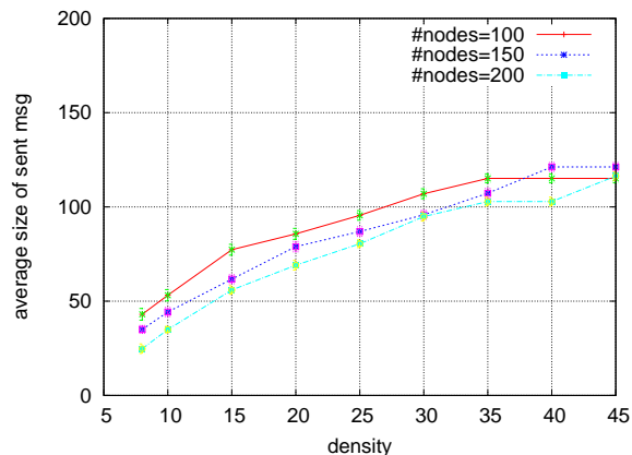
Fig. 6. Average number of bytes sent per node.
