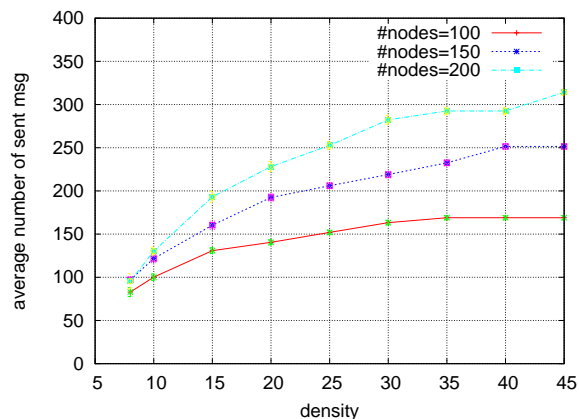
Fig. 5. Average number of messages sent per node.
