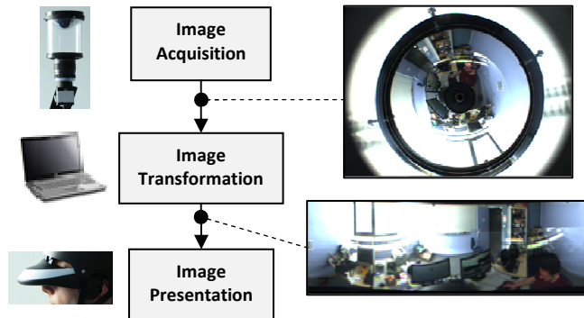
Figure 2: FlyVIZ components
