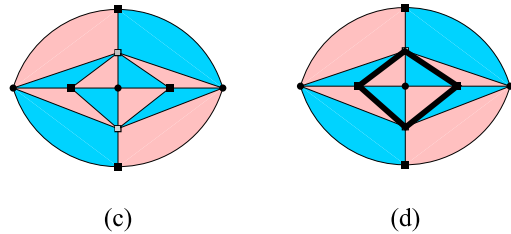
Figure 3. (a) A simplicial poset X . (b) The geometric realization of X . (c) The geometric realization of \text{sd}(X) , which also equals \dot{D}_X(0) . (d) \dot{D}_X(b) is a 1-dimensional simplicial complex that is a cycle of length four (in black bold lines).
