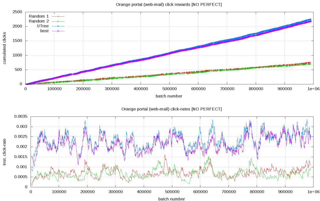
Figure 4: Challenge protocol applied on Orange dataset
