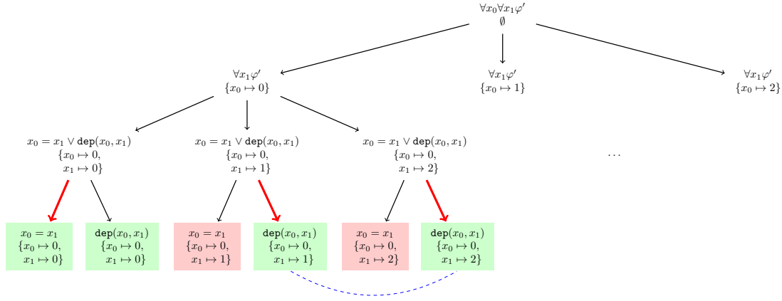
Figure 1: Evaluation game for \forall x_0 \forall x_1 (x_0 = x_1 \vee \mathbf{dep}(x_0, x_1)) with M = \{0, 1, 2\}
