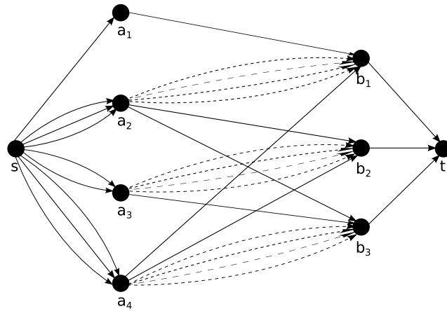
Figure 4: Flow graph D_I constructed from a set F containing the clauses B_1 = (x_1 \vee \bar{x}_2 \vee x_4) , B_2 = (x_2 \vee \bar{x}_3 \vee x_4) and B_3 = (x_2 \vee x_3 \vee \bar{x}_4) . [The example assumes l = 4 . Dashed arcs have capacity \frac{1}{4} . The others have capacity 1].
