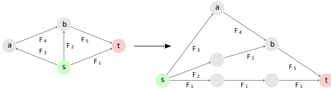
Figure 6: Example of the construction of Theorem 5 Left: \mathcal{D}' . Right: \mathcal{D} . A vertex u is placed at the level L_{\mathcal{D}}(s, v) , with L_{\mathcal{D}}(s, v) the length of a longest path between s and v . Each arc (u, v) \in A is then subdivided into a path of length L_{\mathcal{D}}(u, v) .
