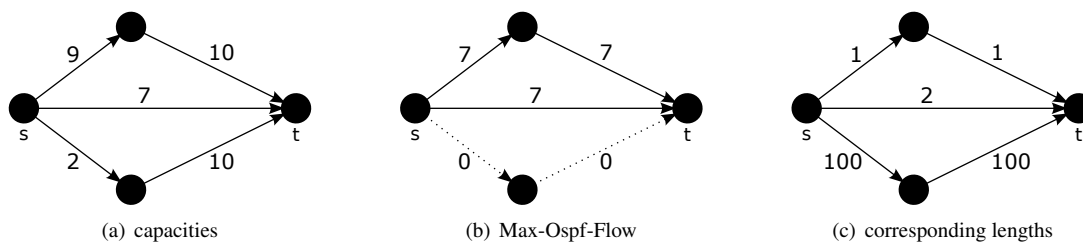
Figure 1: Example of maximum ospf-flow of value 14.
