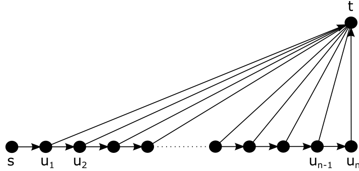
Figure 2: A flow graph with a big gap between Max-Ospf-Flow and the standard maximum flow. Arcs on the path s - u_1 - u_2 - \dots - u_n have all capacities equal to n while arcs entering t have all capacities equal to 1.
