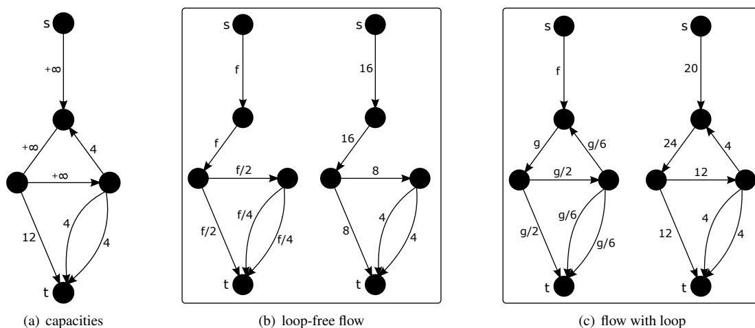
Figure 3: Example of an instance where the optimal flow can only be achieved using a loop: when avoiding the loop, one can easily check that the limitation comes from the constraint f/4 \leq 4 which means that the flow sent from s to t is at most 16; while using a loop the same constraint allows g to be equal to 24 which leads to a flow going from s toward t that is equal to f = g - g/6 = 20 . Other configurations with less arcs are not depicted but lead to even lower ospf-flow value.
