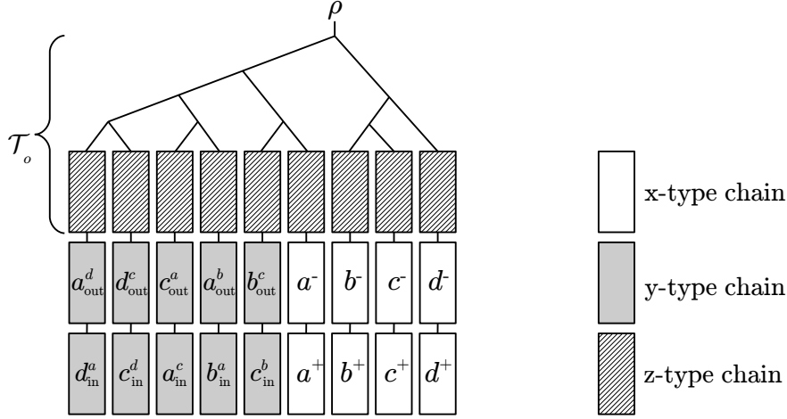
FIG. 5.2. \mathcal{T} : the first tree of the constructed MAAF instance.
