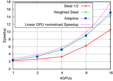
Fig. 5: Speedup (w.r.t. one GPU) when scaling GPUs and using 128 CPUs. r_{\max} = 10 .
