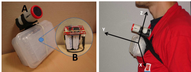
Figure 2: Overview of the device capturing both video and motion. Left: The integrated prototype is composed by a (A) Camsports HDS-720p and a (B) Ultimate IMU board with its battery. Right: The prototype is fixed on an actor's chest and records his motion on 3 axes.
