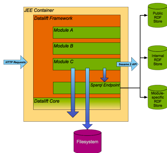
Figure 2: Datalift Architecture
