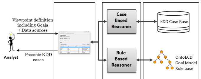
Figure 5. Architecture overview of our implementing tool.
