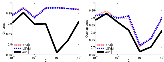
Figure 2. The average test loss over five folds ( y -axis) of the action detection application for different values of C ( x -axis, shown in log-scale). Left: 0/1 loss; Right: Overlap loss. Our framework outperforms both LSVM and ILSVM and provides statistically significant improvements for both types of loss (see text for details).
