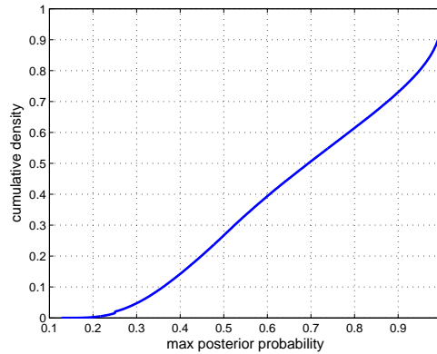
Figure 2: Cumulative distribution of the max of the posterior probability \gamma_k^* = \max_k \gamma(k) on PASCAL VOC 2007 for SIFT descriptors.
