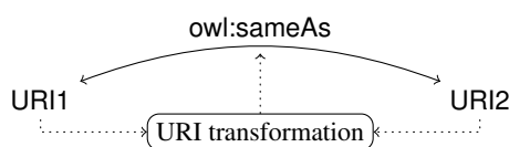
Figure 2: URI transformation.
