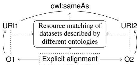
Figure 7: Two datasets matched using an explicit alignment.
