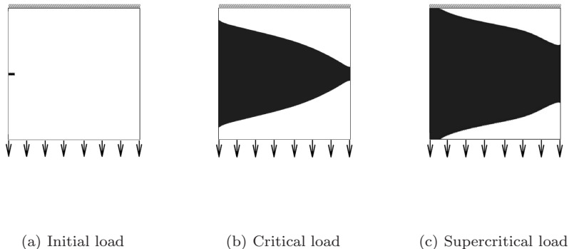
Figure 1: Mode I damage for the 320 \times 320 mesh with 100 time steps. Initial configuration with an imposed displacement of 0.02 (a) critical load at an imposed displacement of 0.06 (b) and supercritical load with an imposed displacement of 0.072 (c).
