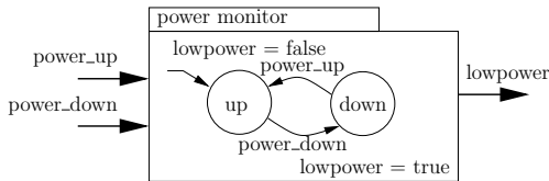
Figure 4: Component power-monitor.
