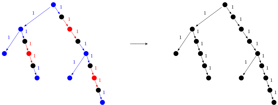
Figure 7: \mathcal{T}_2 and \mathcal{T}_2^{unco} in the proof of Theorem 3.
