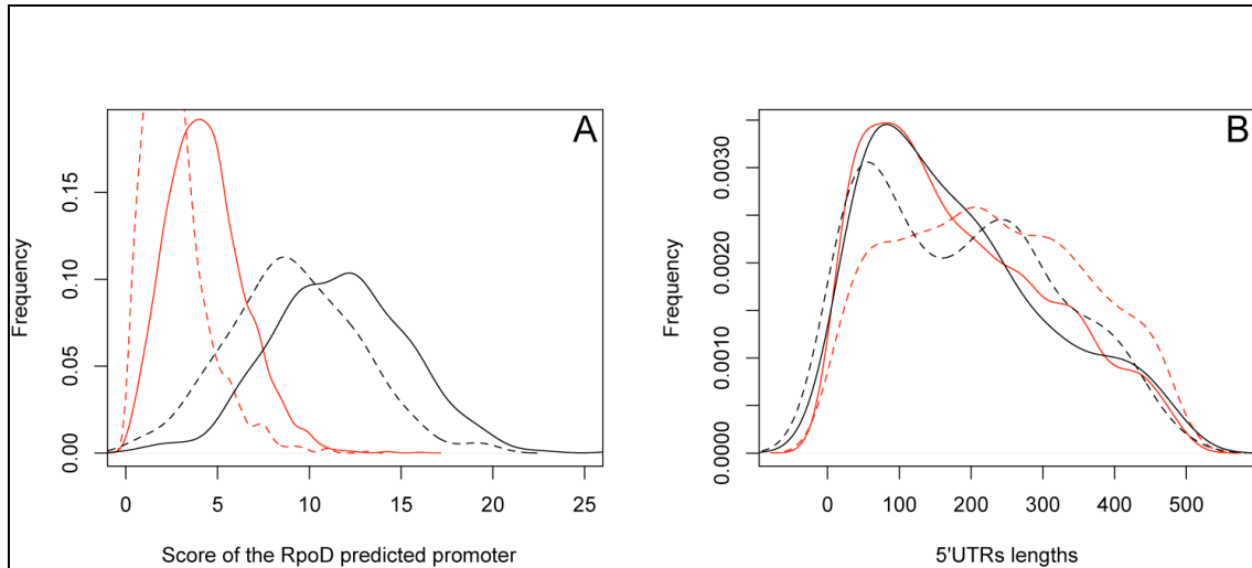
Additional file 5. Distribution of \sigma^{70} prediction scores and 5'UTR lengths in BAp and E. coli . (A) Distribution of \sigma^{70} prediction scores in BAp (black) and E. coli (red) at the beginning of transcription units (continuous lines) and within transcription units (dotted lines); (B) Distribution of the size of the predicted 5'UTR. Scores and UTR lengths are calculated by BPROM.
