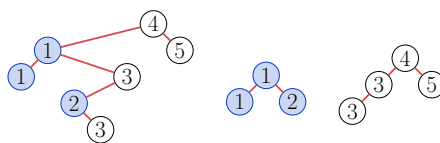
Figure 3: A right binary search tree T , T_{\leq 2} and T_{>2} .
