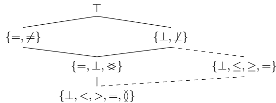
Fig. 2. The reasonable weakenings of A_5 ( \not\perp = \{<, >, =, \emptyset\} and \cong = \{<, >, \emptyset\} ).
