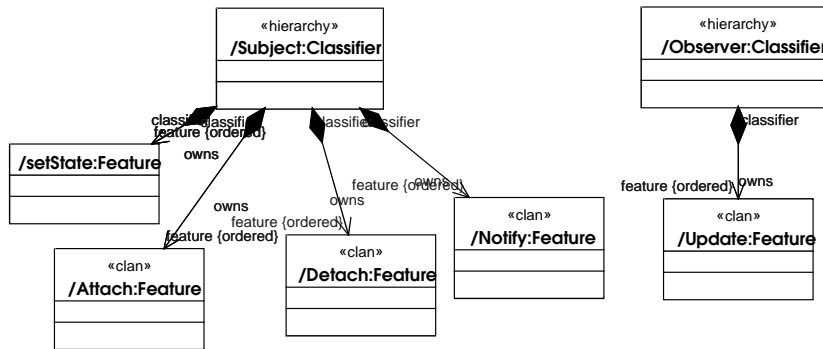
Fig. 2. Meta-level collaboration of the Observer design pattern
