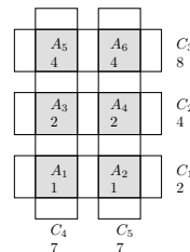
Fig. 5. Selecting two conformers by the greedy strategy fails to report the optimal solution. The shaded regions have the weights as indicated and the unshaded regions have null weights.
