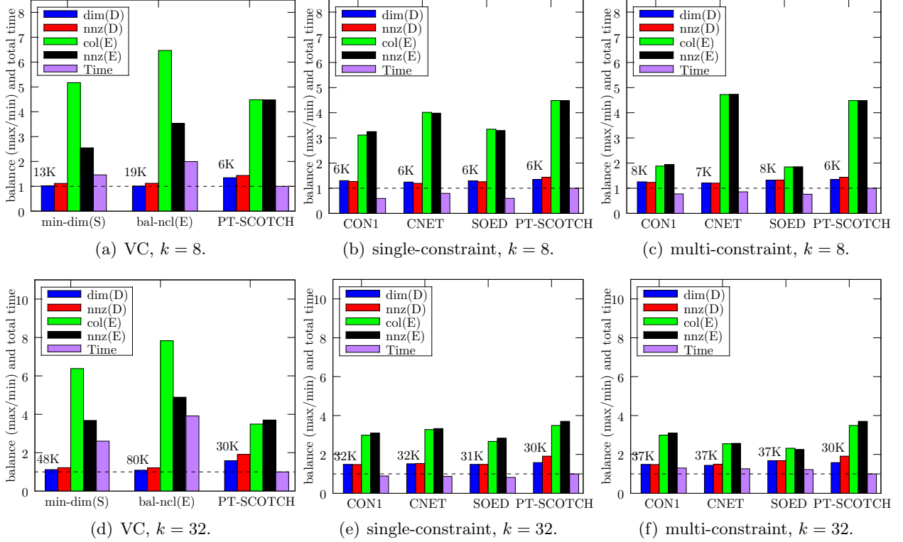
Figure 1: Load balancing and solution time with matrix tdr190k . In the legend, “dim( D )” refers to the dimension of D_\ell , “nnz( D )” refers to the number of nonzeros in D_\ell , “col( E )” refers to the number of nonzero columns in E_\ell , “nnz( E )” refers to the number of nonzeros in E_\ell , and “time” refers to the total runtime of PDSLIn. The number on top of each group of bars is the separator size.
