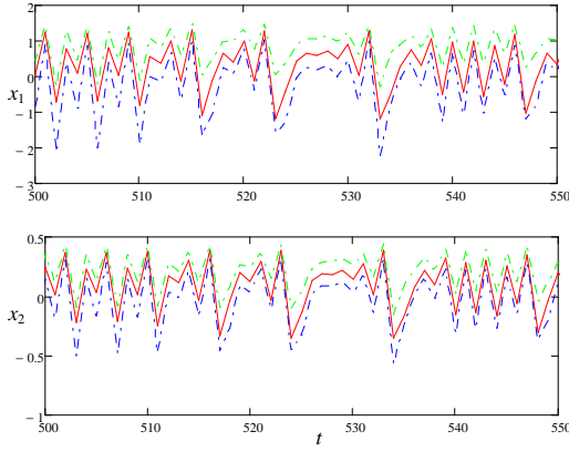
Figure 2. The results of simulation for Lorenz model
