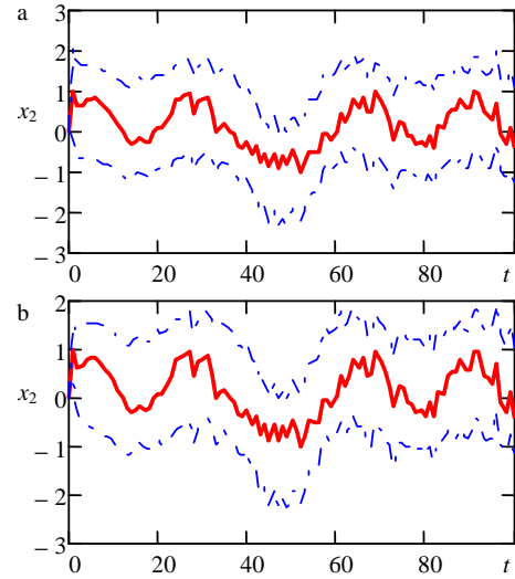
Figure 1. Comparison of interval estimation performed by the observer (4) (part (a)) and (5) (part (b))
