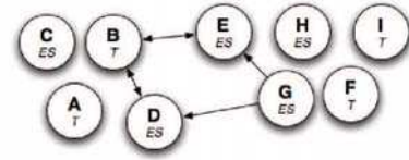
Figure 3: Argumentation framework
