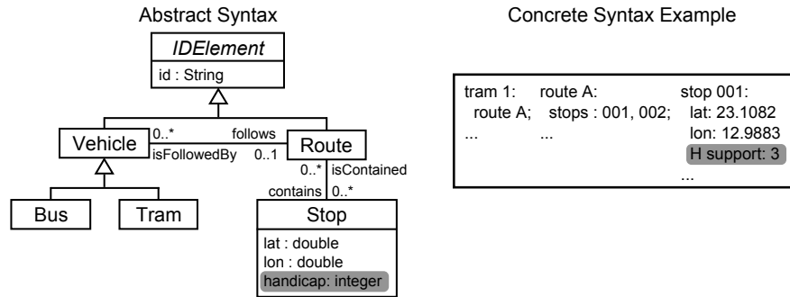
Fig. 1. Abstract syntax and an example of concrete syntax of the Transport DSML (grey-filled boxes represent elements added after the collaboration).
