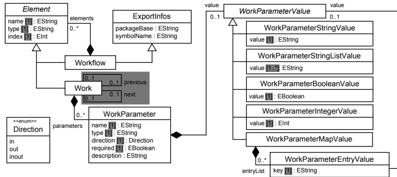
Fig. 8. Abstract syntax of the MDRE workflow language (grey-filled boxes show the changes of the resulting abstract syntax).
