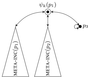
Fig. 16: The action e_M(k, l, m) when I_k = \text{inc}(0) . The case I_k = \text{inc}(1) is by replacing p_2 and p_3 everywhere.
