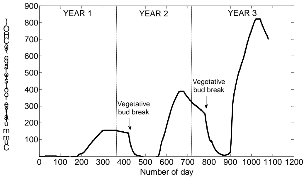
Fig 7. Seasonal variations of total carbohydrate reserves in the root during three consecutive years of peach tree growth. The simulated tree was trained to a perpendicular V system. In the third year, crop load was 100 fruits tree -1 . Abbreviations: CHO = carbohydrates.
