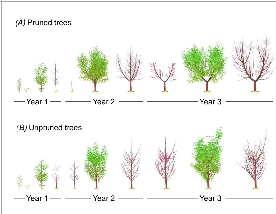
Fig 3. Model output showing three-dimensional depiction of a pruned peach tree (A) and an unpruned peach tree (B) over three years of growth. The pruned tree was trained to a perpendicular V system by means of pruning cuts in winter. The final tree height was about 3.0 m.
