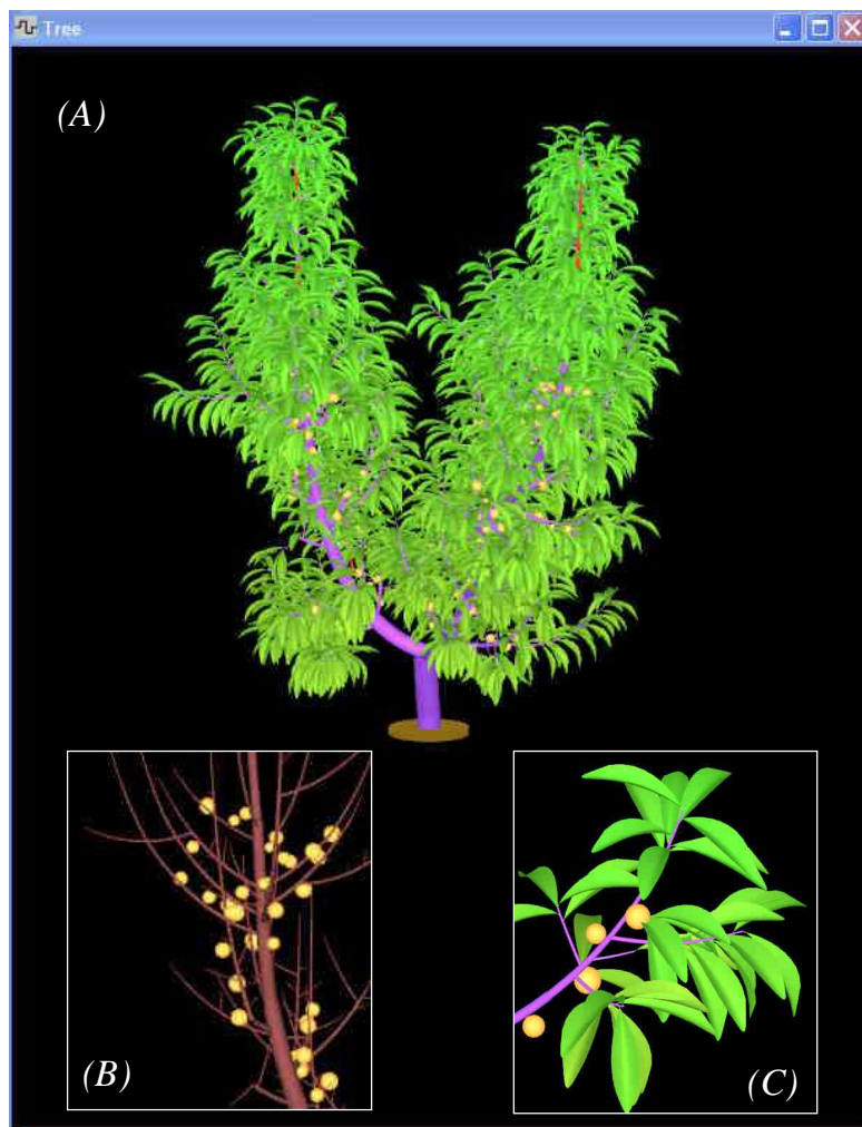
Fig 1. L-studio output showing the potential of L-PEACH to simulate three-dimensional structure of mature peach trees (A), and intra-canopy variability among organs of the same type in response to localized source-sink behaviors (B, C). L-studio also allows modifications in the property that is visualized by the stem's colors, i.e. , movement of carbohydrates through the tree (A,C) (see Allen et al. 2005 for further details on carbohydrate fluxes and colors), or a bark-like color (B). In Figure 1B, leaves were removed to increase visibility of fruit.
