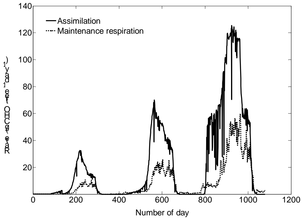
Fig 5. Simulated seasonal patterns of daily carbohydrate assimilation and maintenance respiration during three consecutive years of peach tree growth. The simulated tree was trained to a perpendicular V system. In the third year, crop load was 100 fruits tree -1 . Abbreviations: CHO = carbohydrates.
