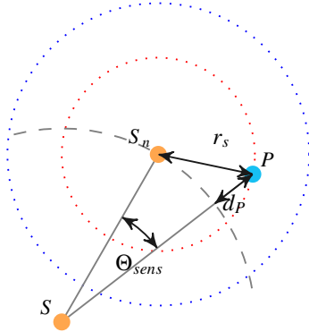
Figure 6: The difference between angular coordinates of sensor S_n and the PoI P_i in the moment when sensing begins.
