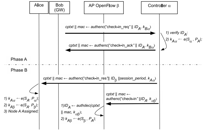
Fig. 4. Authenticated key-agreement.
