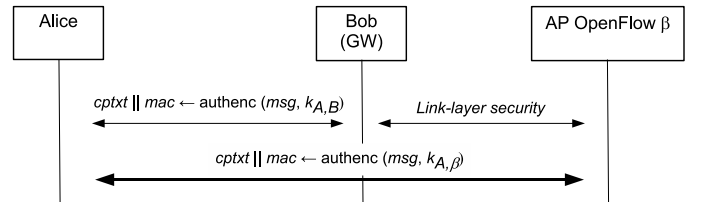
Fig. 6. End-to-end security.
